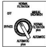
SELECTOR SWITCH DETAIL
